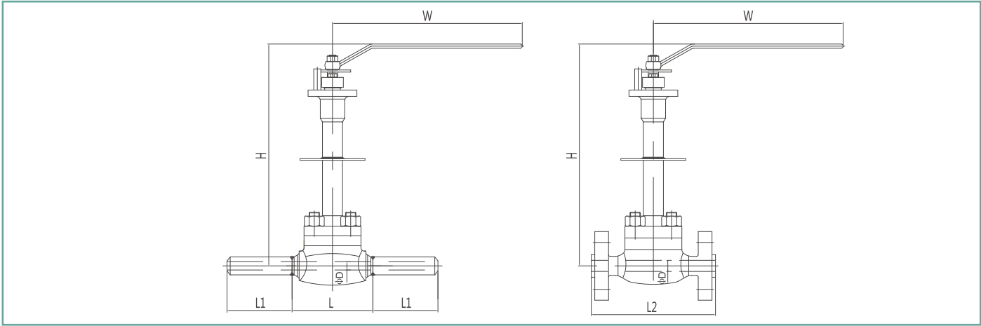
Class 150 / 300 / 600
